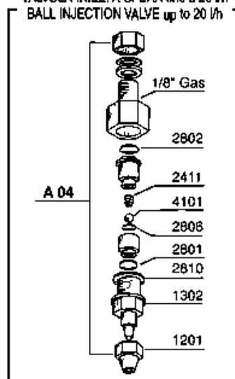
VALVOLA INIEZ. A SFERA fino a 20 l/h BALL INJECTION VALVE up to 20 l/h
