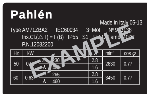
B. Rating plate for a pump motor.
