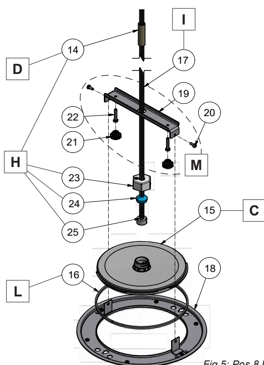
Fig 5: Pos 8 LED Light unit assembly
